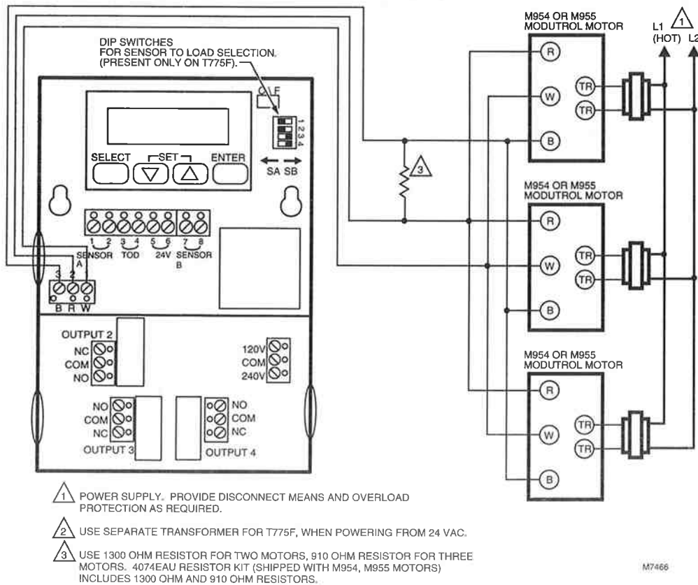
Fig. 16—Wiring T775 with up to 3 Series 90 Modutrol Motors.
