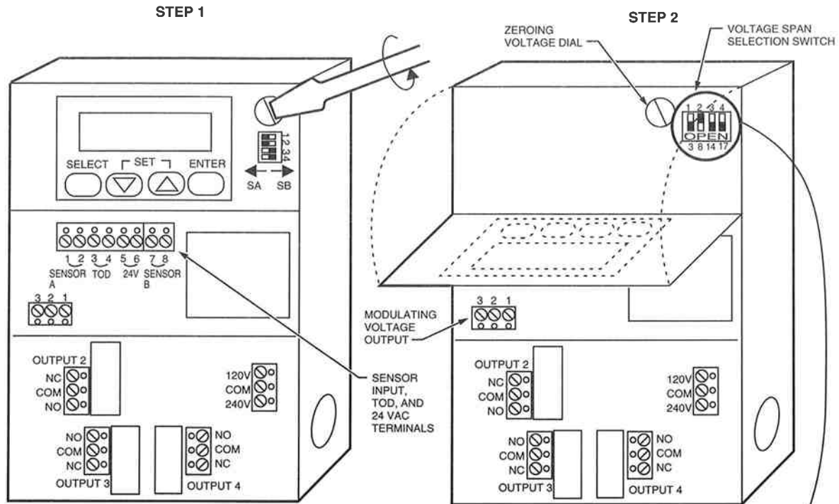
Fig. 22—Output voltage span selection.
