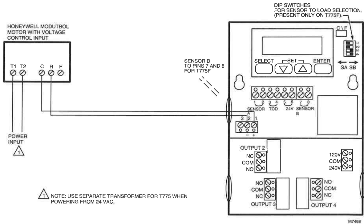
Fig. 18—Wiring T775 with modulating actuator with voltage control input.
