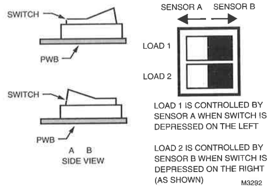
Fig. 23—DIP switch settings for sensor selection.
