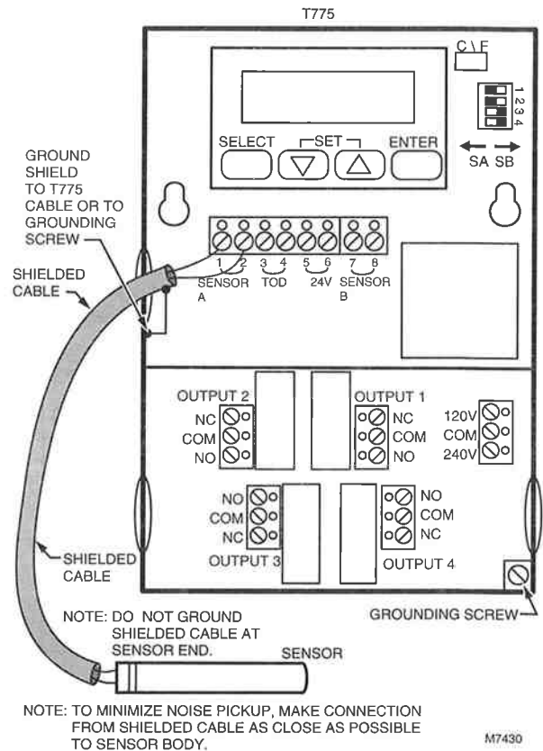
Fig. 5—Using shielded cable for cable runs longer than 25 feet.
