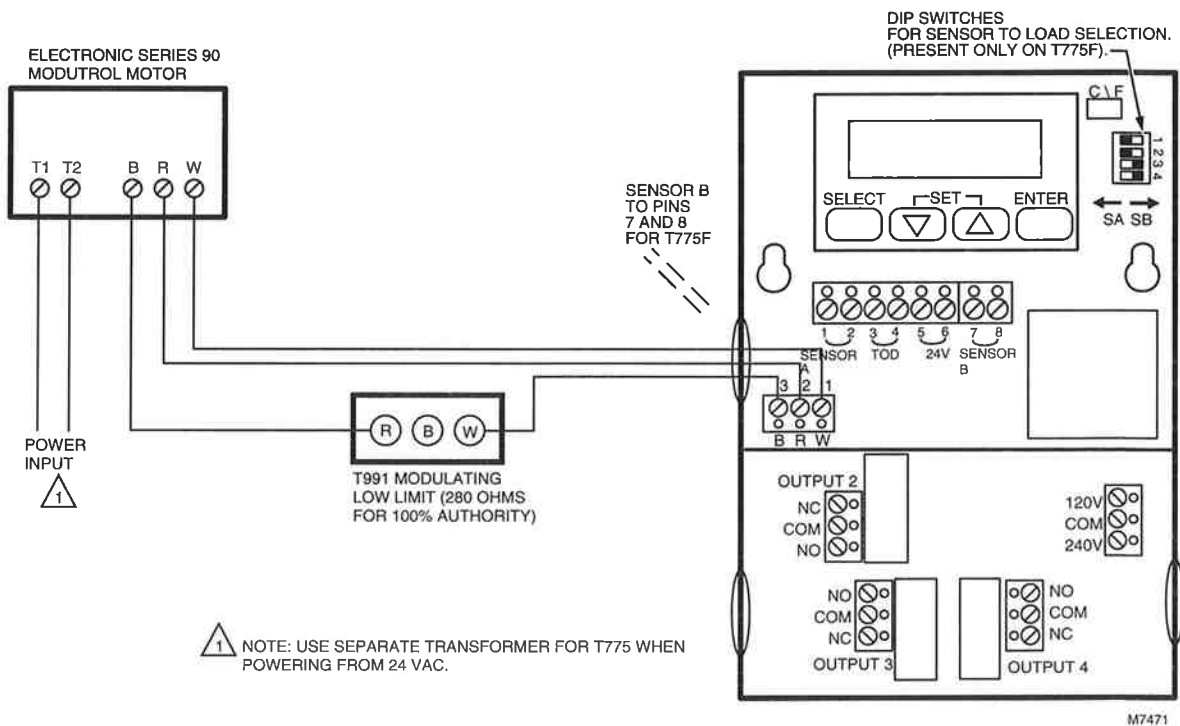
Fig. 14—T991 used with Series 90 Modutrol Motor and T775 to provide modulating low limit.
