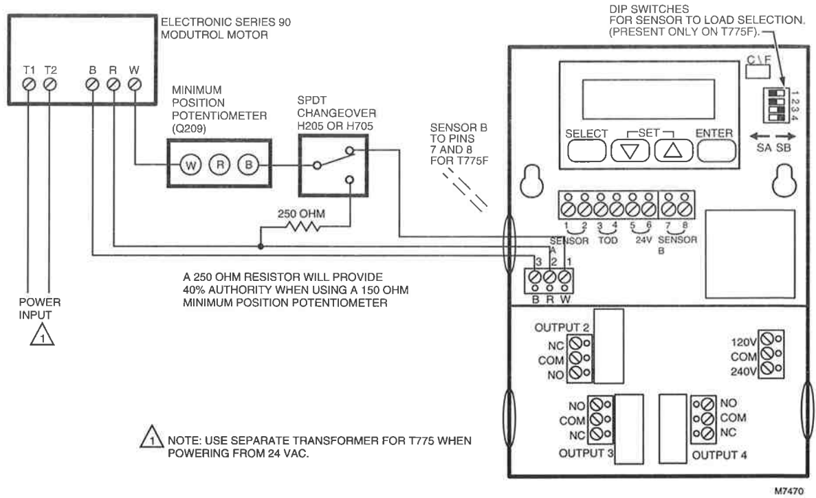
Fig. 13—Changeover relay and minimum position potentiometer used with Series 90 Modutrol Motors.
